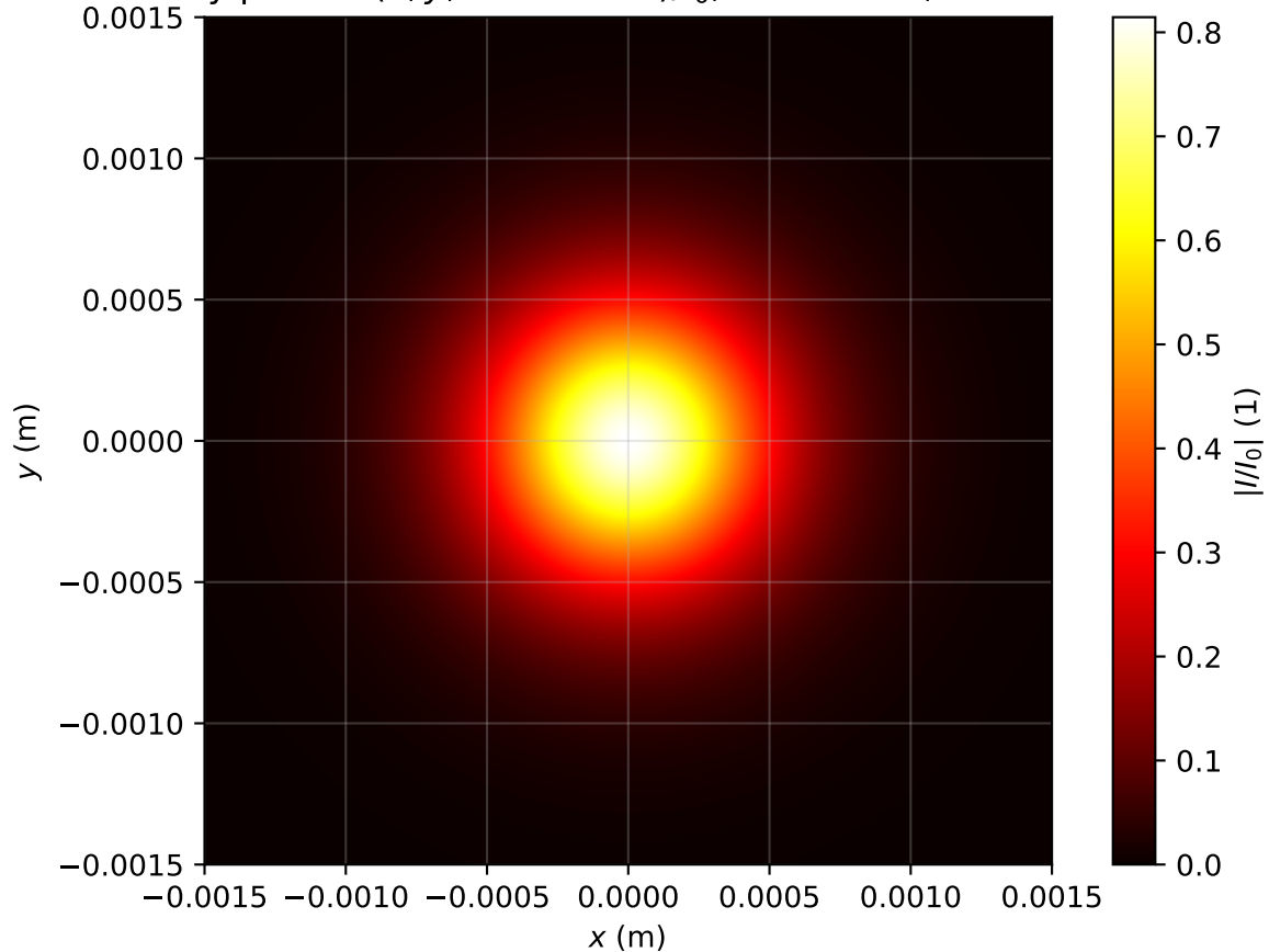
Intensity profile I(x, y, z = 3.105m)/I_0 , Pin=0.7Pcr, artificial time
